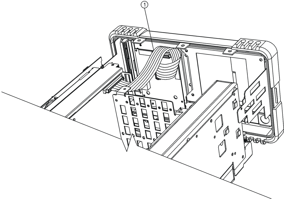
Figure 19 Front Frame Ribbon Cable
