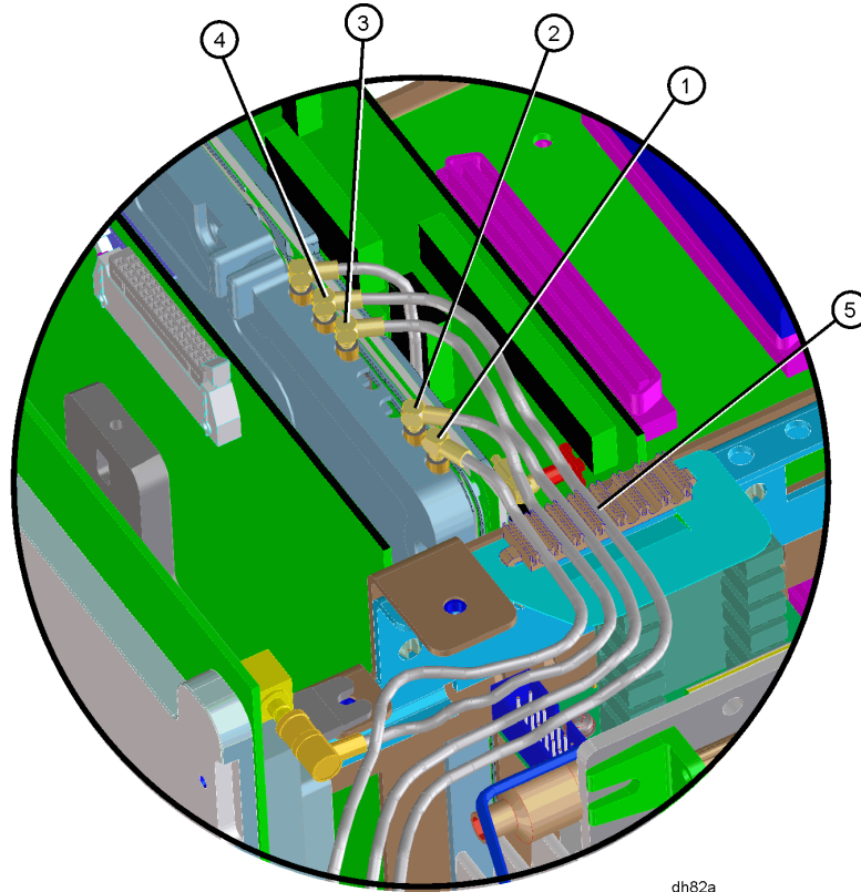
Figure 14 Cable Connections to A7A8 DDRF Assembly
