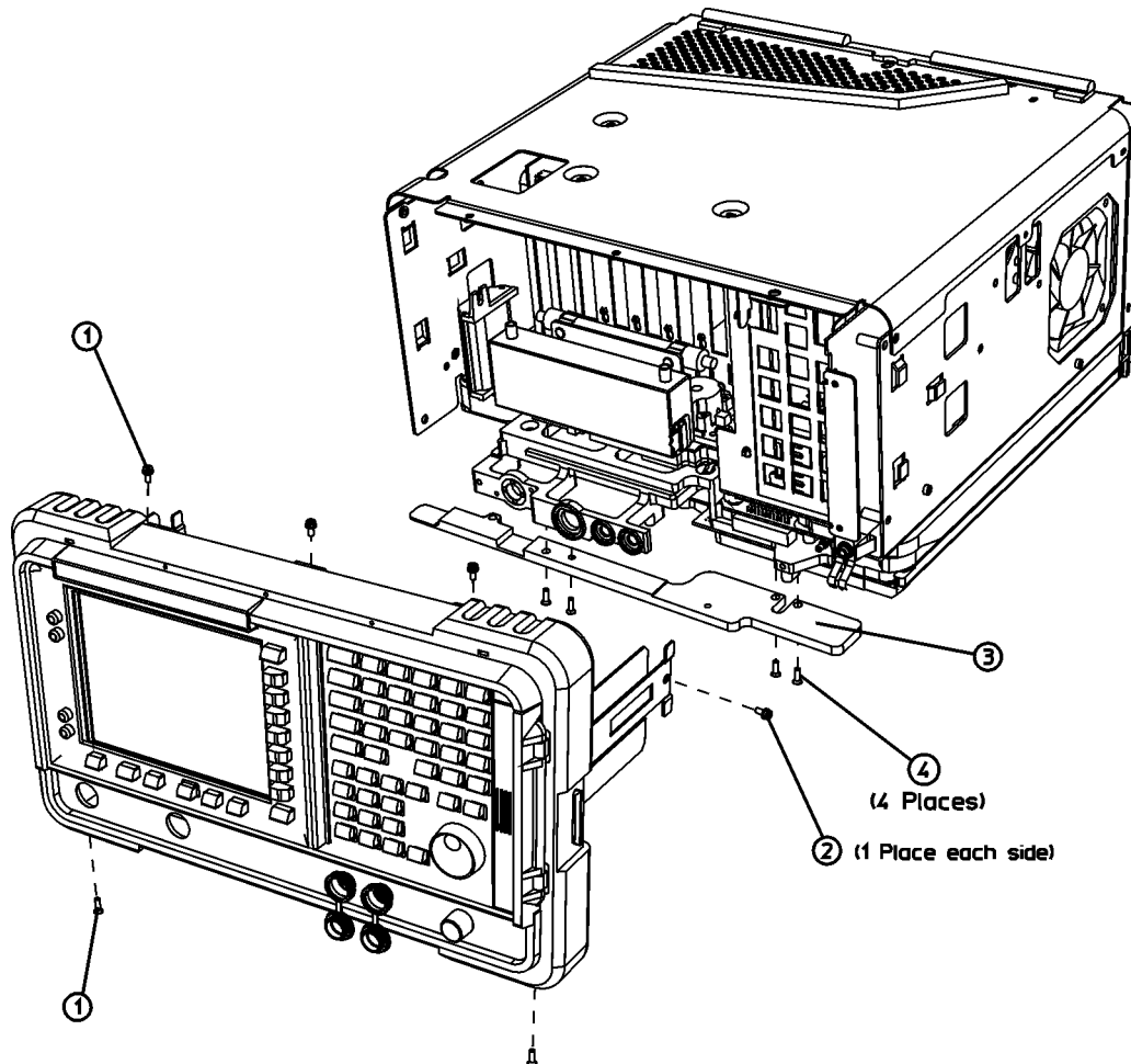
Figure 18 A1 Front Frame Assembly Replacement
