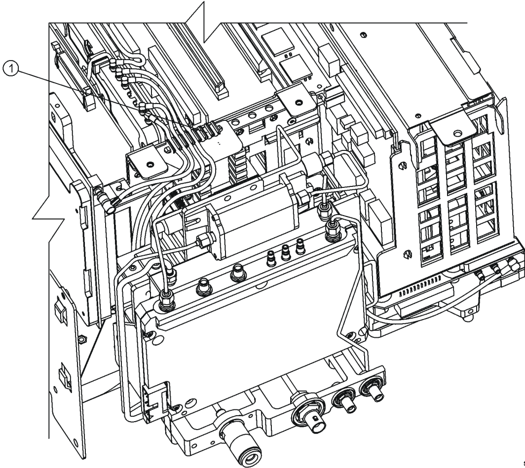
Figure 8 Digital Demod RF Assembly Cable Clip
