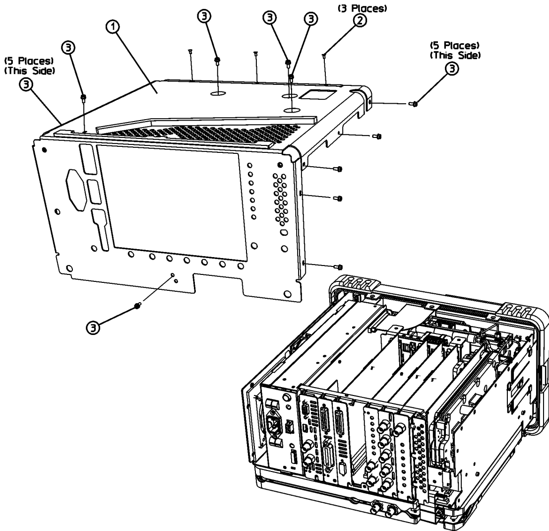
Figure 20 Inner Shield Replacement
