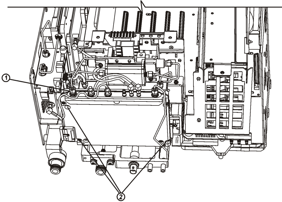
Figure 17 Re-installing the LO Amplifier/IF Switch Assembly
