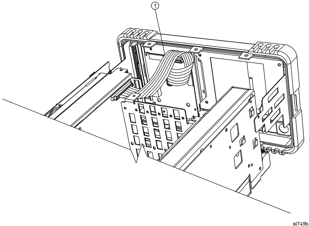
Figure 4 Front Frame Ribbon Cable
