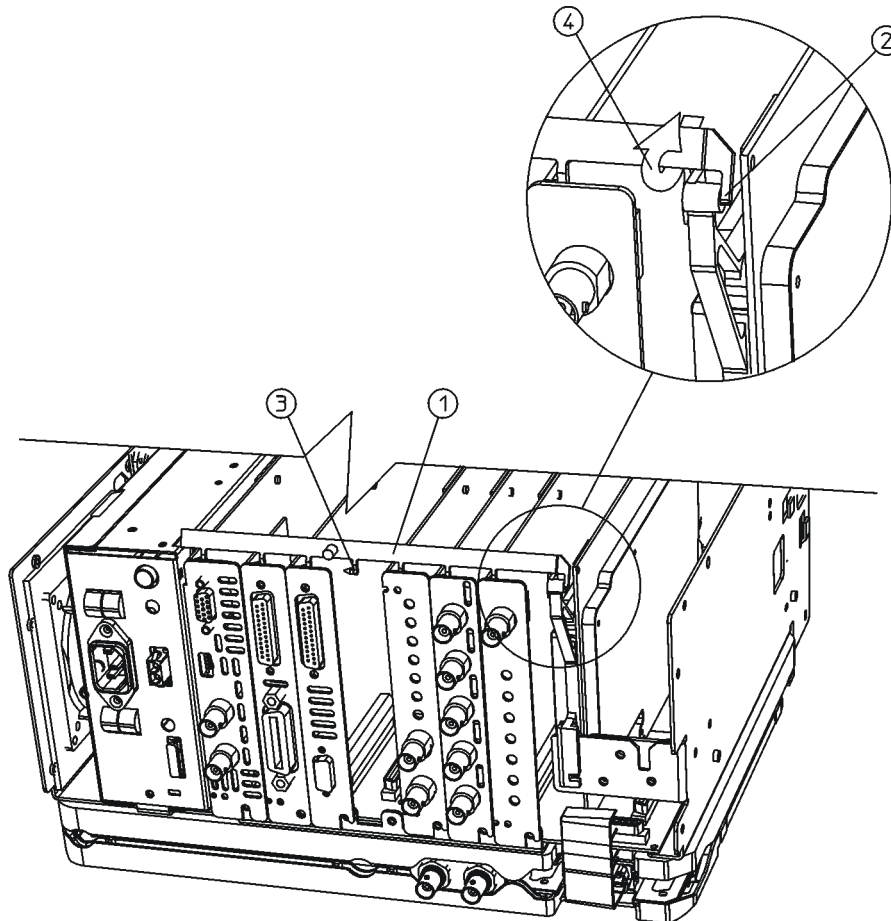
Figure 15 Installing the Vibration Support Bar
