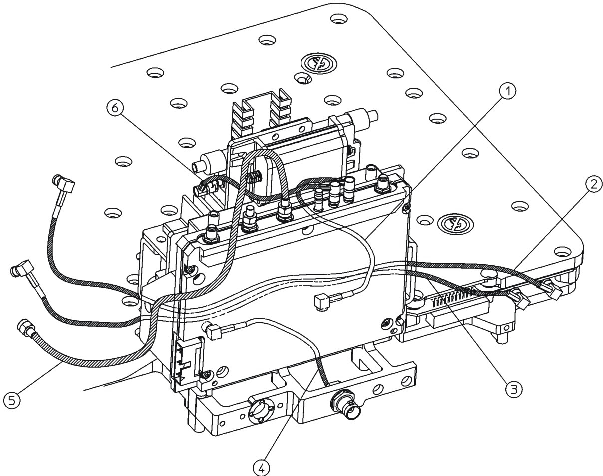
Figure 6 Original Cable Identification and Routing
